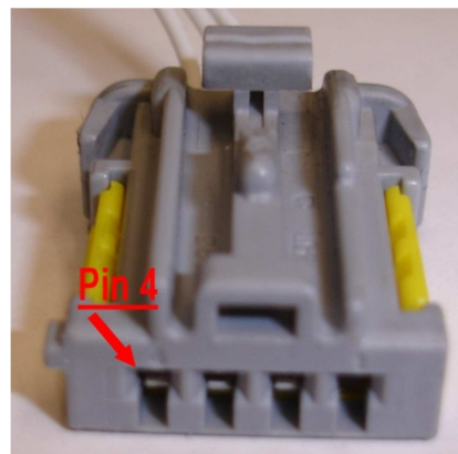
Ring decoder connector shown disconnected Pin 4
